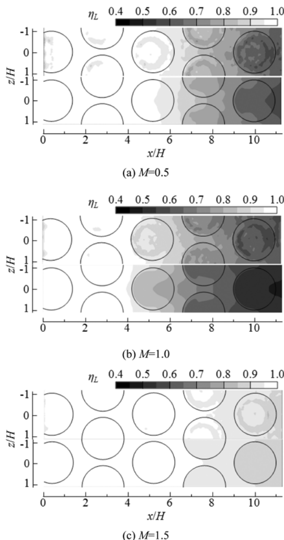
Fig. 3 Contour of local film cooling effectiveness, \eta_L , of experiments 9) (upper half) and LES (lower half) for spherical dimple.
