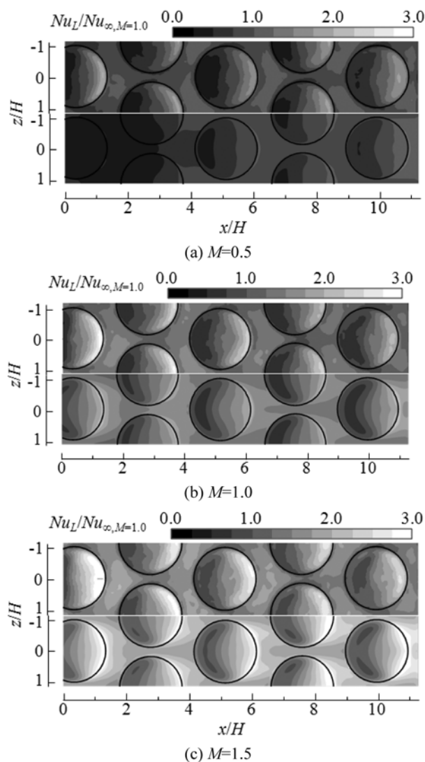
Fig. 5 Contour of local Nusselt number, Nu_L/Nu_{\infty, M=1.0} of experiments 9) (upper half) and LES (lower half) for spherical dimple.
