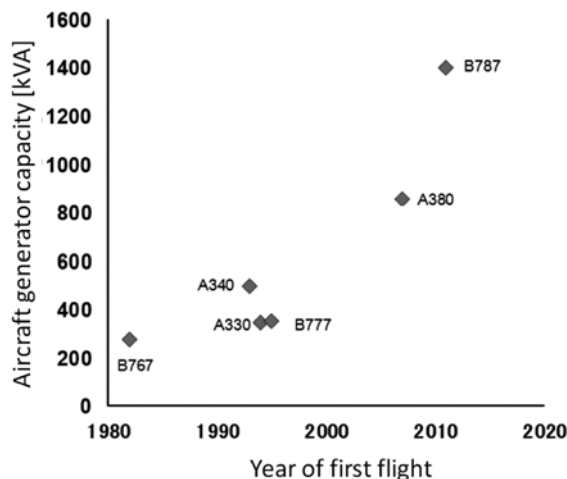
Fig. 1 Commercial aircraft generator capacity trend.
