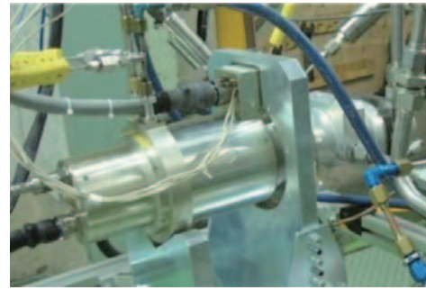
Fig. 8 The electric motor-driven fuel pump with a two channel redundant motor
