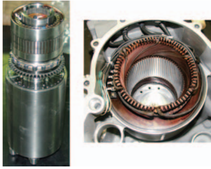
Fig. 1 Two Pole Generator Rotor and Stator
