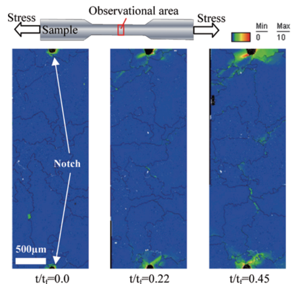
Fig. 4 Intragranular misorientation maps of crept specimens (13) .
