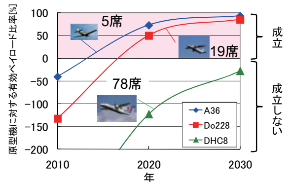
Fig. 5 Feasibility of electric aircraft
