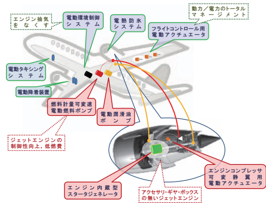
Fig. 1 Concept of the AEA
