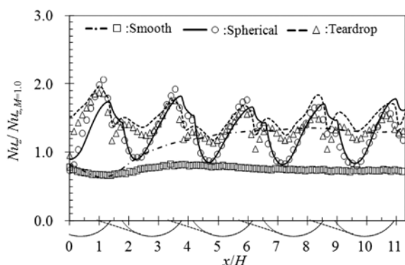
Fig.11 Streamwise distribution of laterally averaged Nusselt number, Nu_z/Nu_{\infty, M=1.0} , for M=1.0 . (Lines and symbols are for LES and experiments 13) , respectively.)
