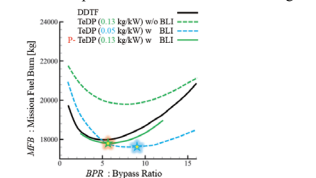
Fuel Burn Analysis of Turbo-Electric Propulsion System
