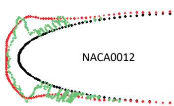
(b) Predicted Ice Shape under SLD Icing Condition
