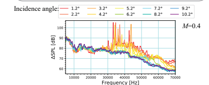
Compressor Noise Spectrum for Various Incidence Angles
